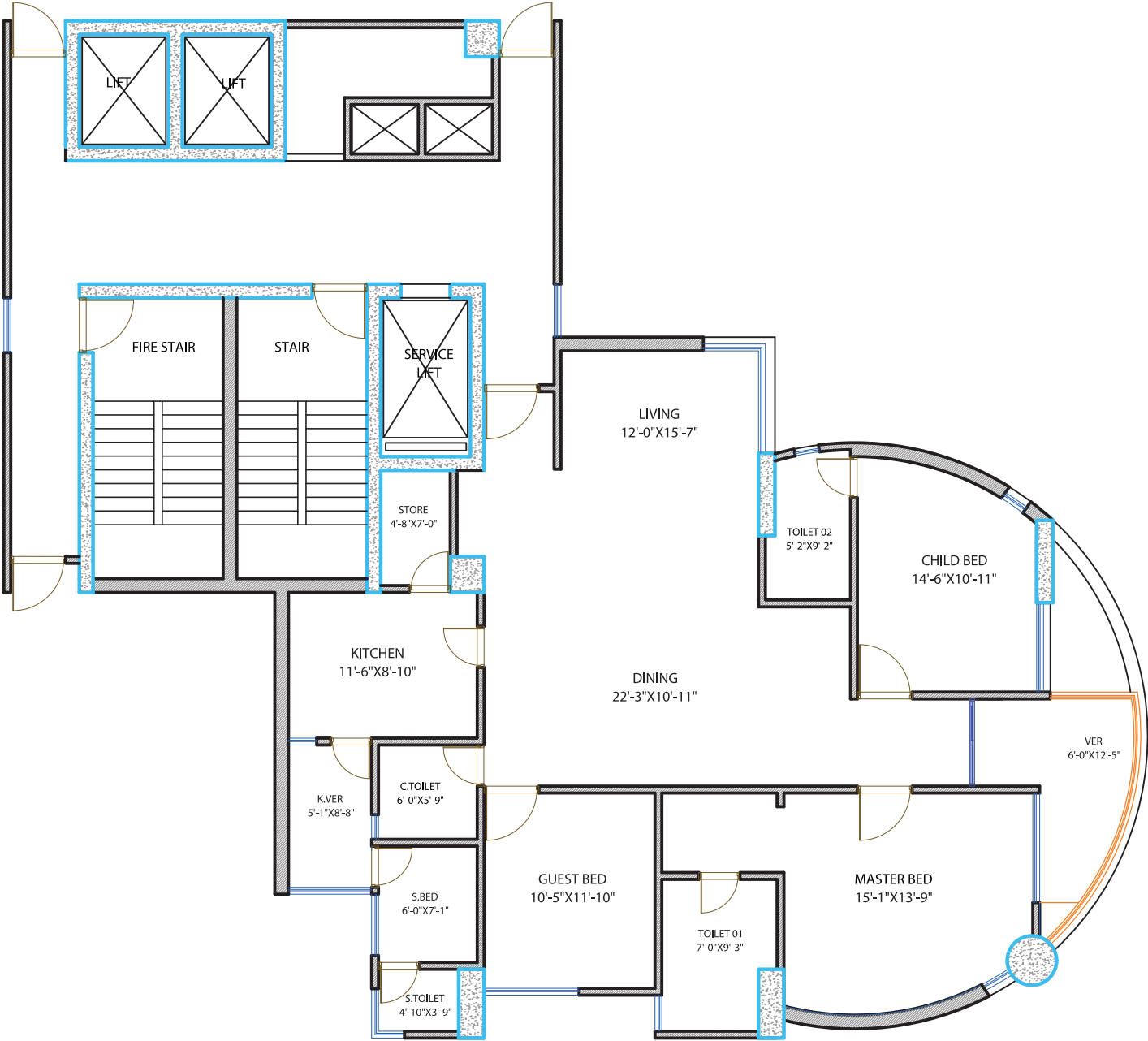
SHANTA GARDEN FLOOR PLAN
