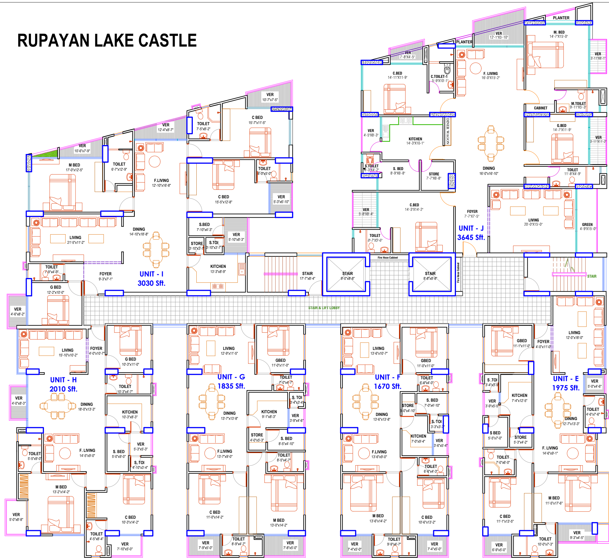
TYPICAL FLOOR PLAN BUILDING - 02
